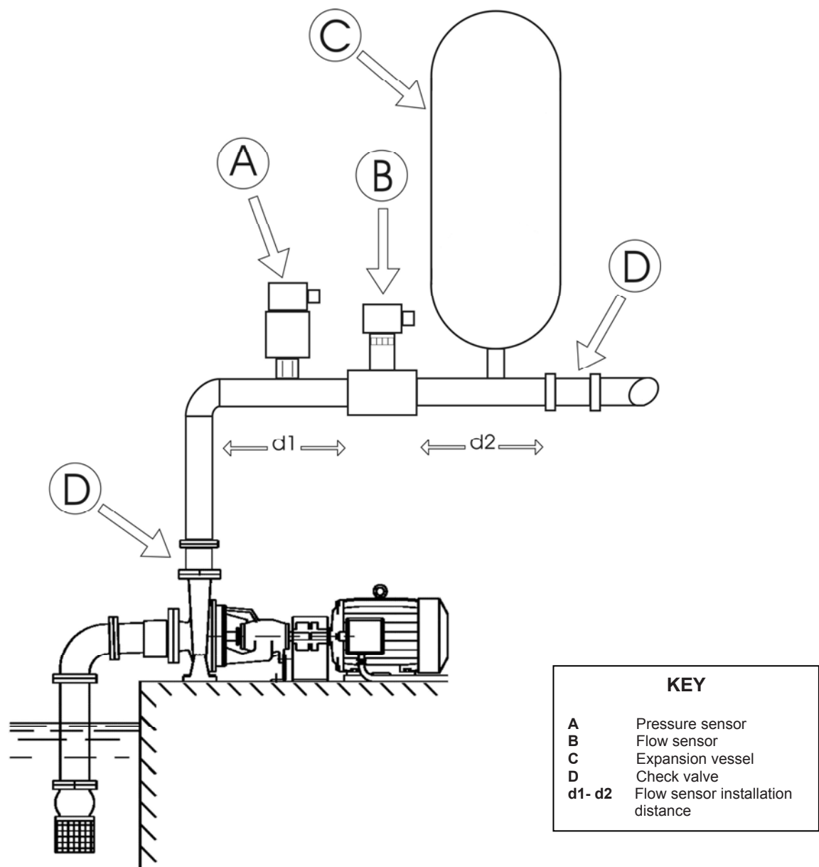
Figure 4: Hydraulic installation
