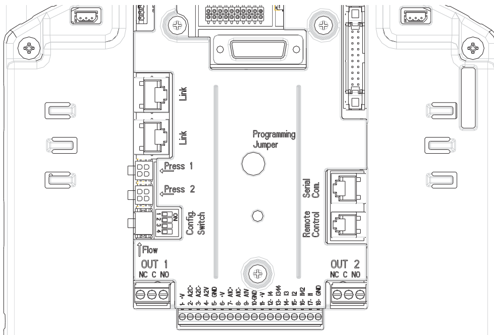
Figure 5: Connections
