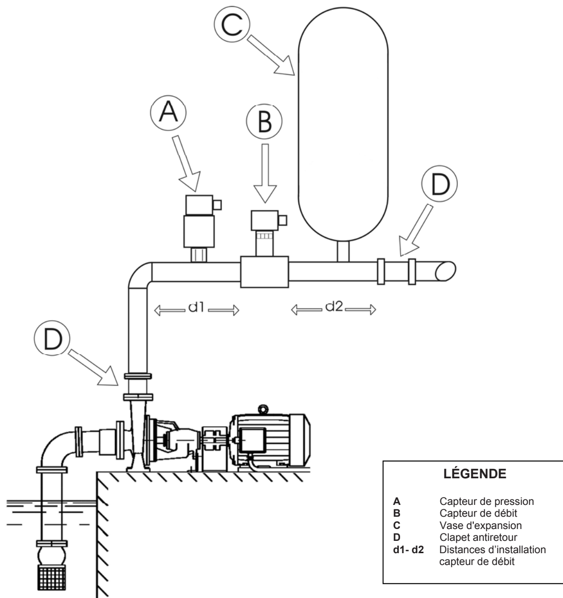
Figure 4: Installation hydraulique
