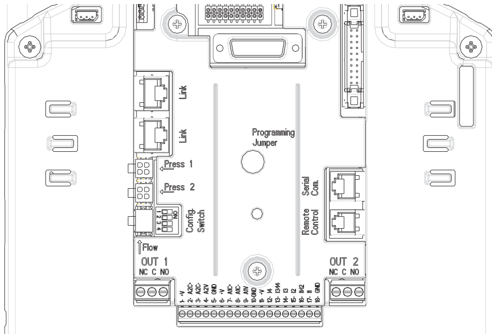
Figure 5: Connexions
