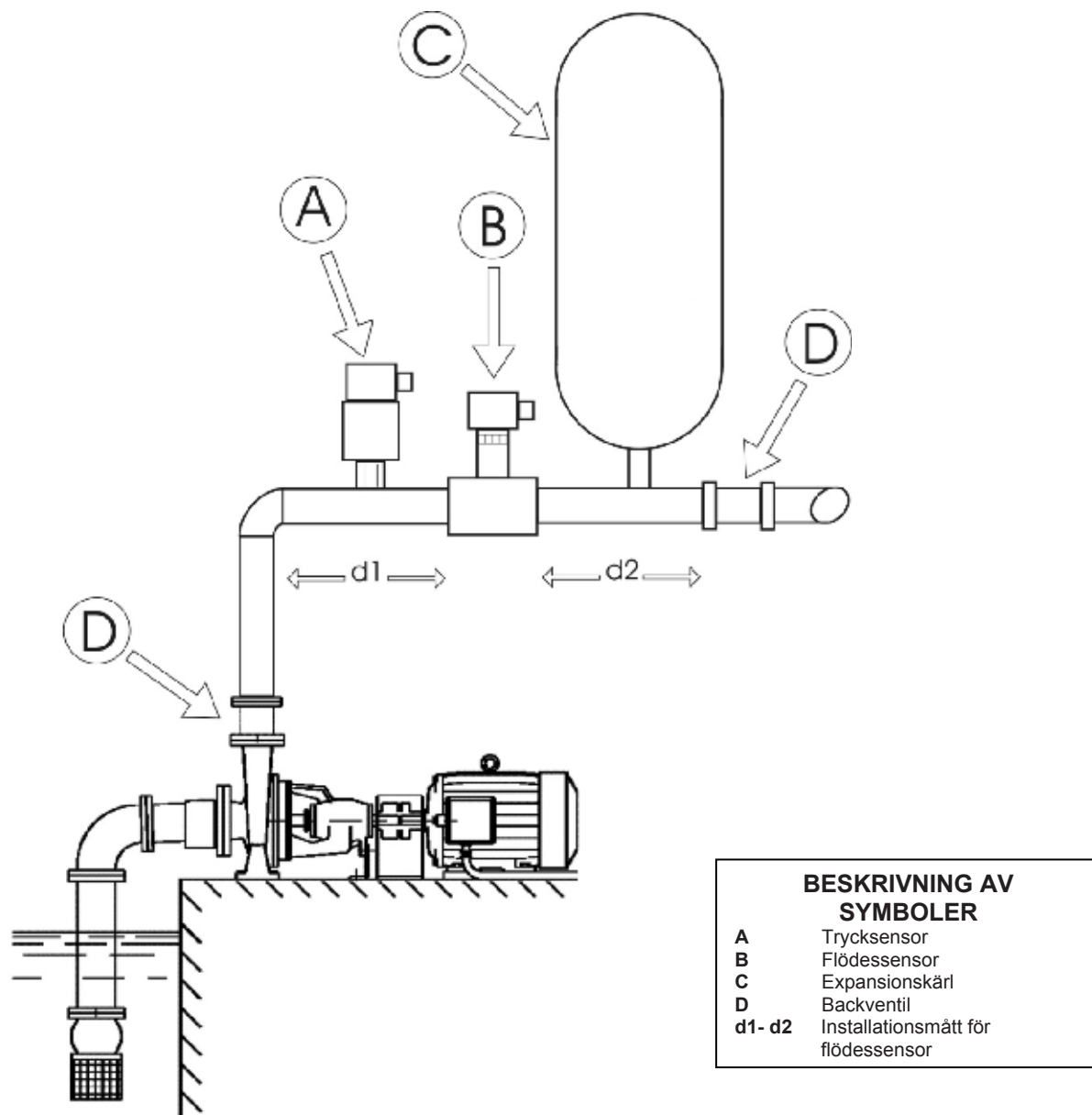
Fig. 4: Hydraulisk installation
