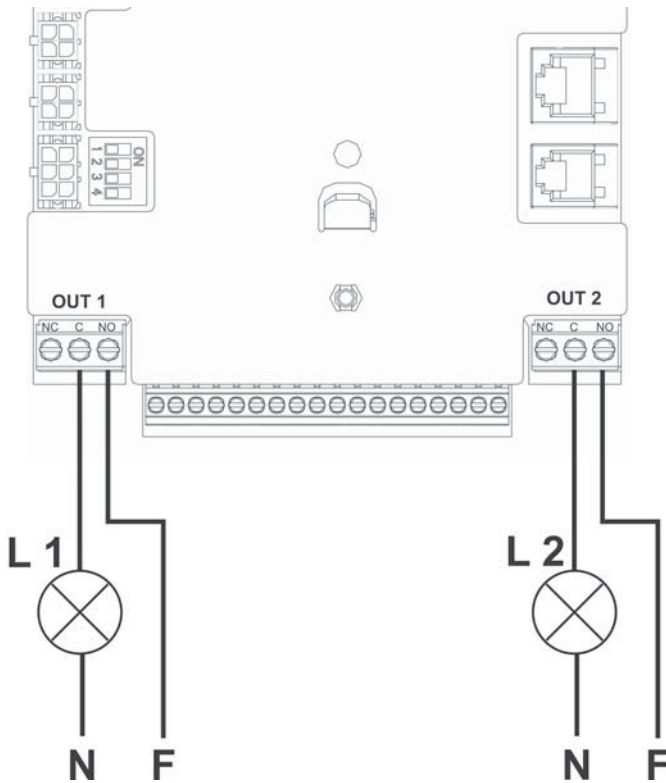
Figure 10: Example of output connections
