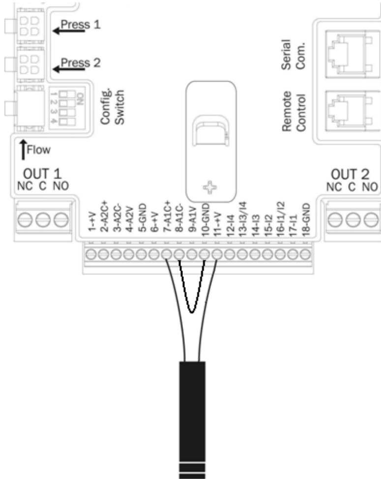
Figure 8: Connecting the 4 - 20 mA pressure sensor
