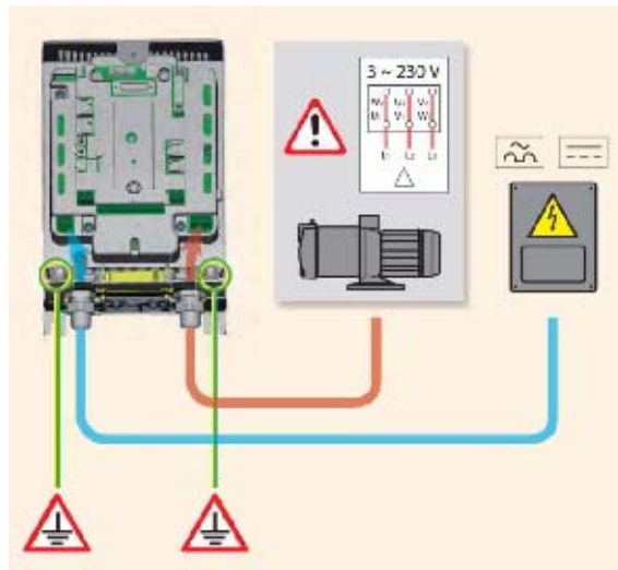
Figure 5: Connexion pompe AD 2.2 AC - 1.5 AC - 1.0 AC
