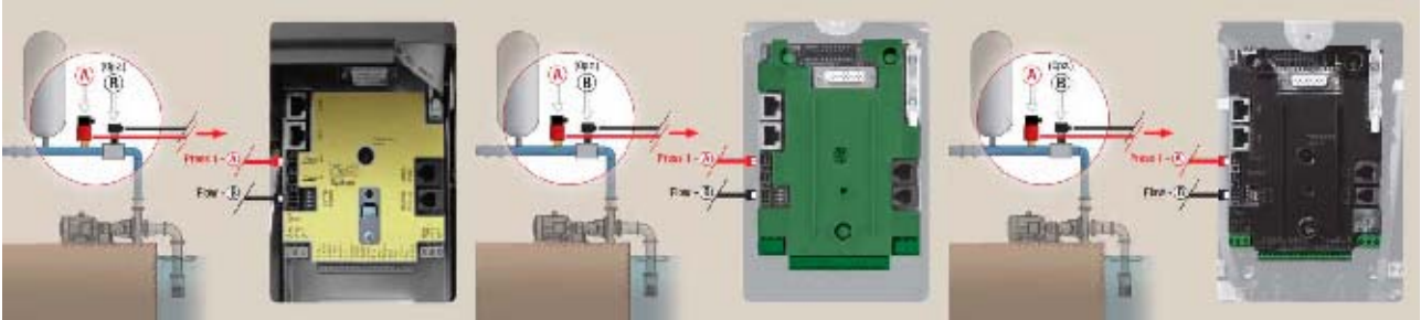
Figure 7: Sensor connections
