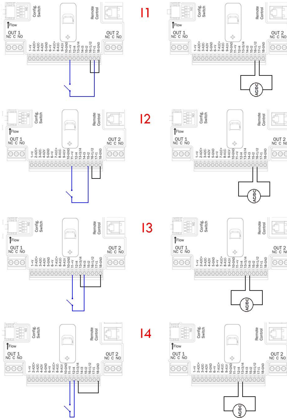
Figure 11: Example of input connections
