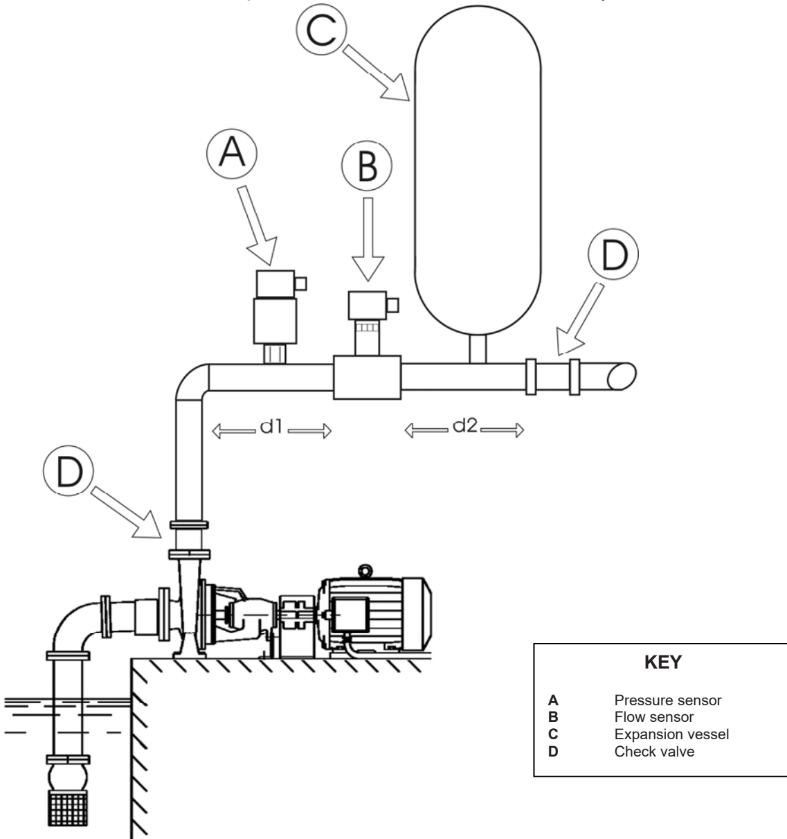
Figure 6: Hydraulic installation
