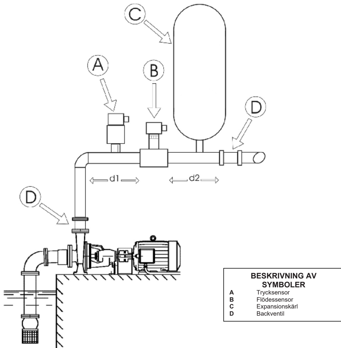
Fig. 6: Hydraulisk installation
