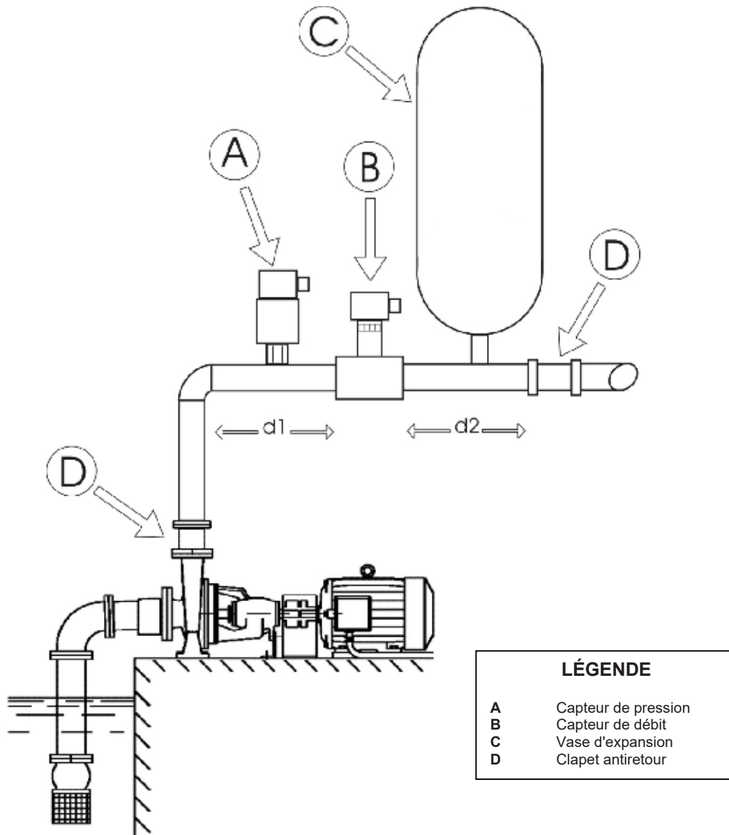
Figure 6: Installation hydraulique
