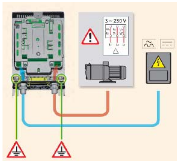
Figure 5: Pump connection AD 2.2 AC - 1.5 AC - 1.0 AC
