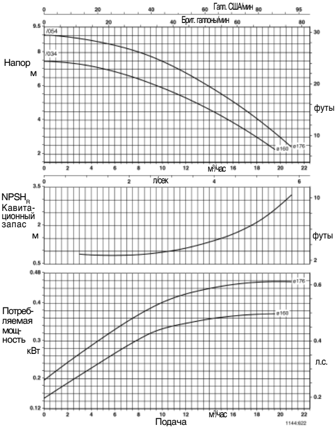
Trialine Z 50-160
