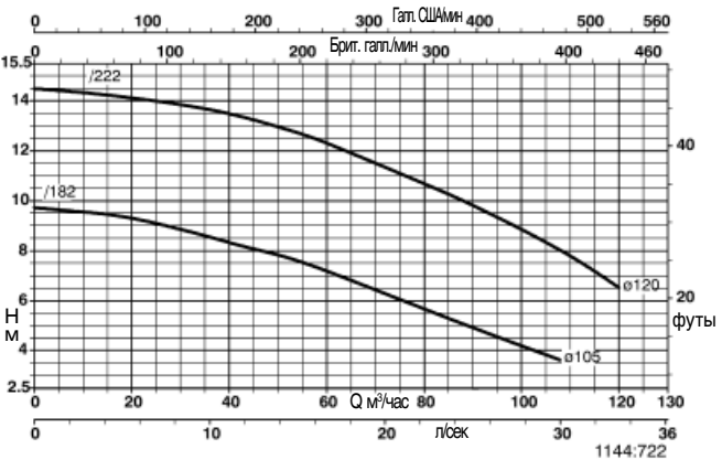
Trialine Z 80-125
