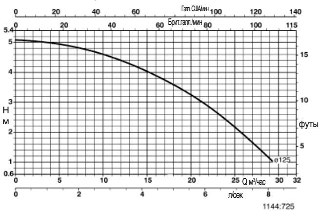
Trialine Z 50-160/054
