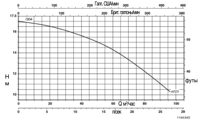
Trialine Z 65-250
