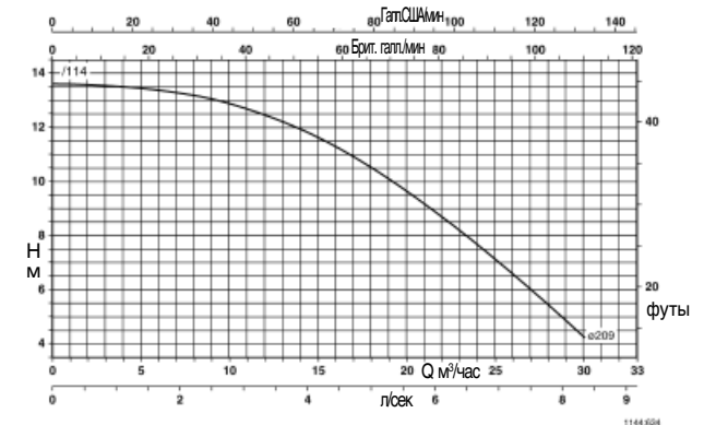
Trialine Z 32-200
