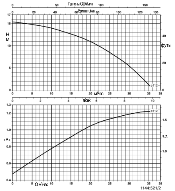
Trialine Z 40-125/132
