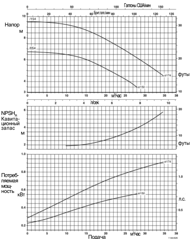
Trialine Z 50-160
