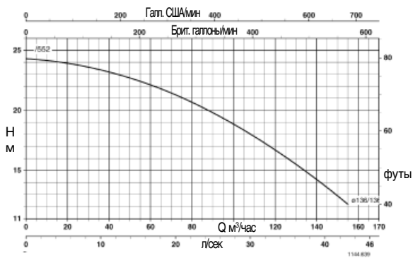
Trialine Z 80-160
