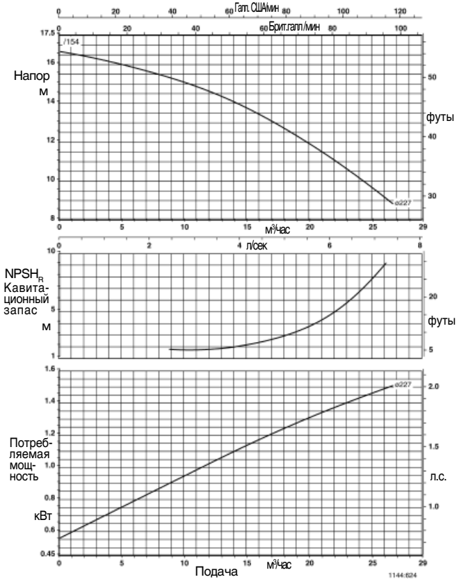
Trialine Z 50-250
