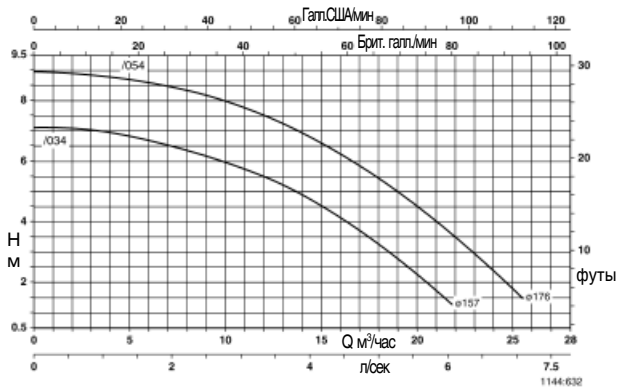
Trialine Z 32-160
