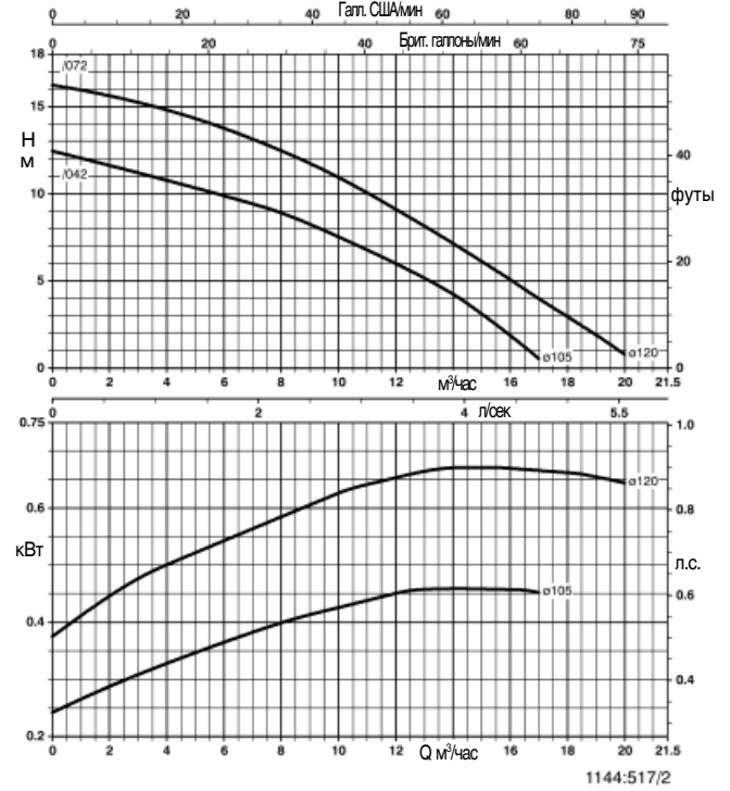
Trialine Z 32-125
