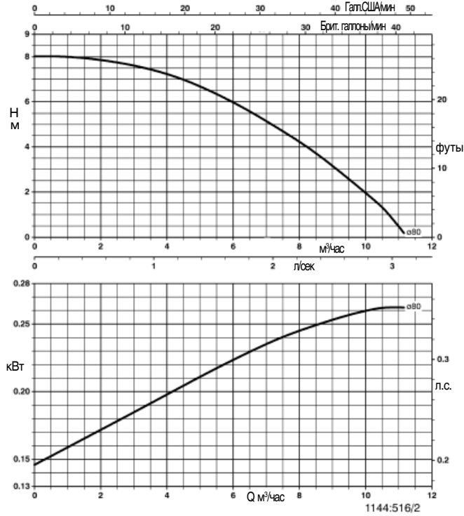
Trialine Z 32-100/022
