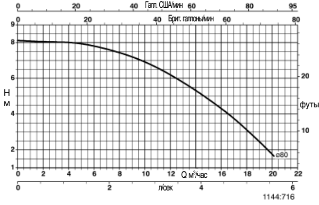
Trialine Z 32-100/022
