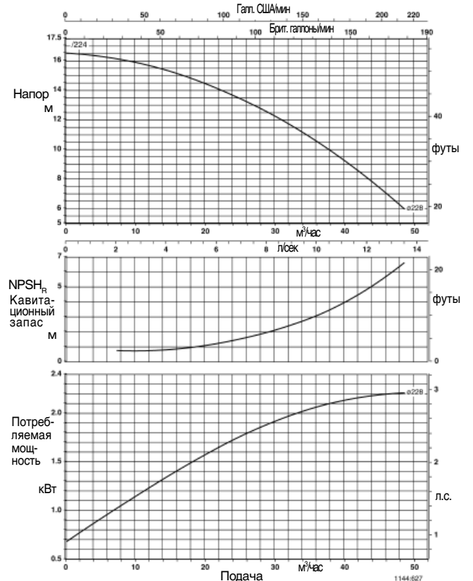
Trialine Z 50-250
