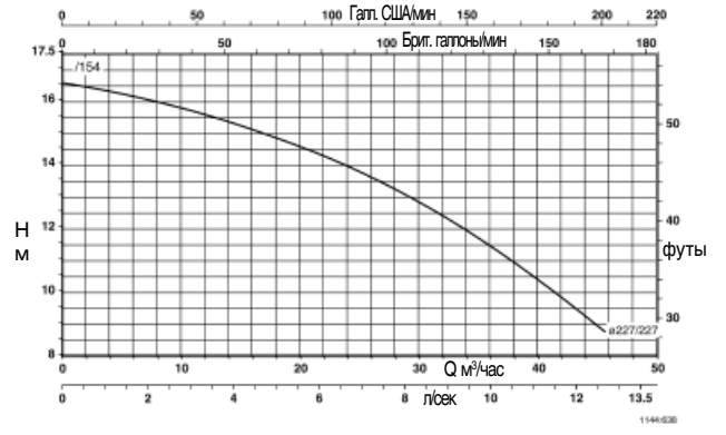
Trialine Z 50-250
