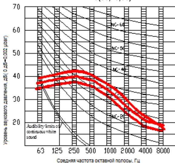
MVC28(36,45,56)A-VA1
