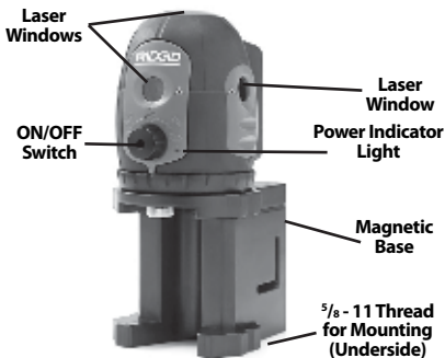
Figure 2 - Laser Parts
