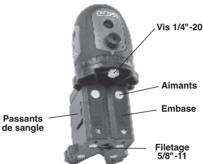
Figure 6 Embase
