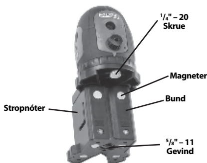
Figur 6 – basis
