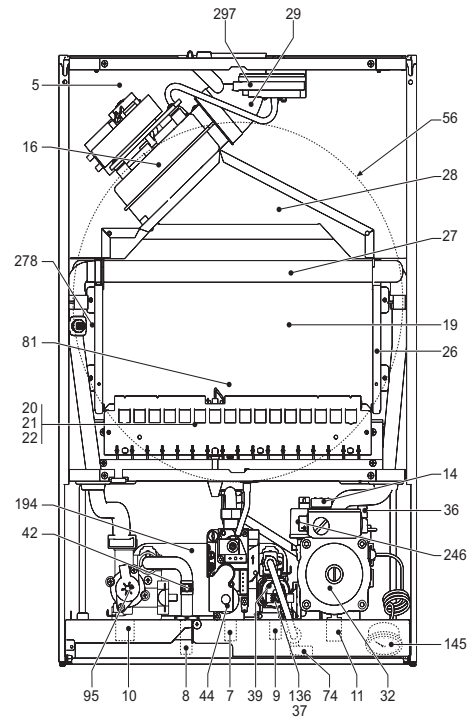
fig. 32 - Vista general DIVAtop MICRO F 37
