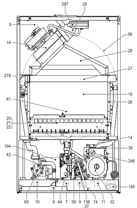
fig. 32 - General view DIVAtop MICRO F 37
