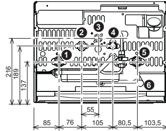
fig. 17 - Plumbing connections
