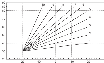
fig. 14 - Compensation curves
