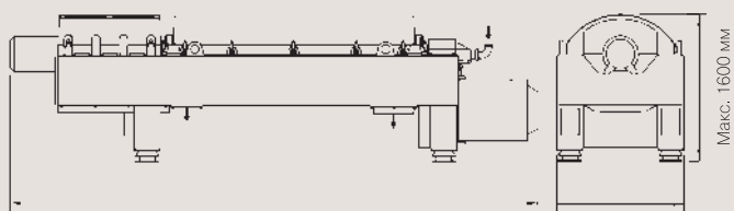
ALDEC G2-60 4550 mm 1110 mm ALDEC G2-70 5000 mm 1110 mm ALDEC G2-80 5035 mm 1200 mm ALDEC G2-100 5665 mm 1300 mm
