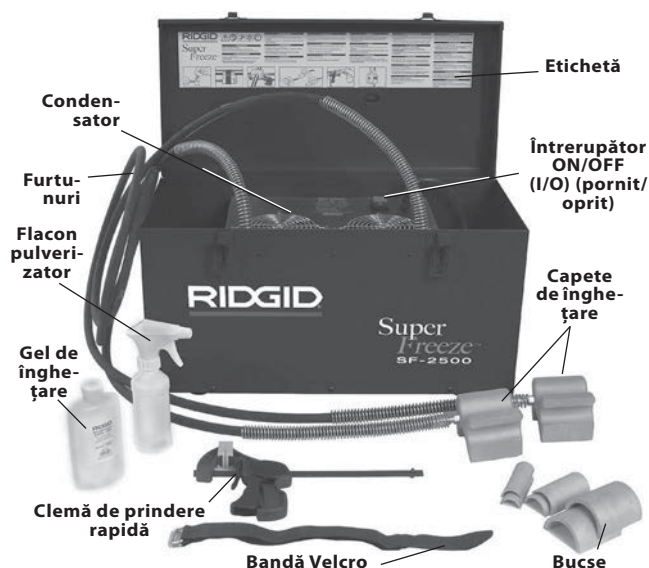
Figura 1 – Unitate SF-2500 SuperFreeze
