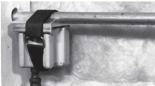
Figure 7 – Freeze Head with End Adapter Attached with Velcro Strap
