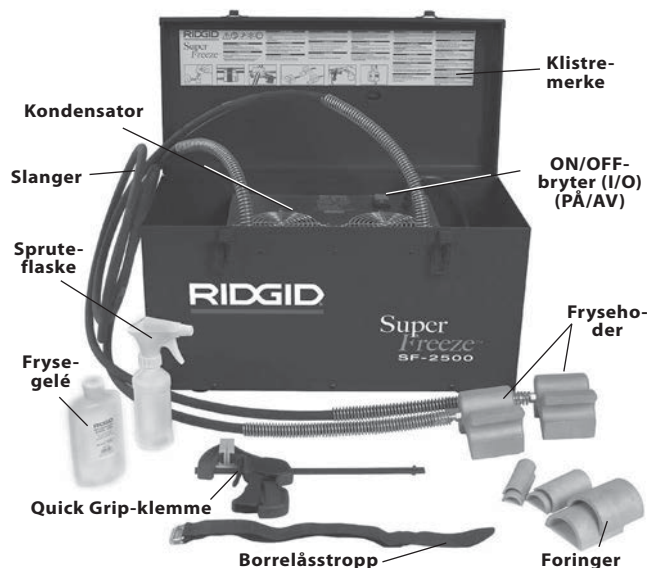
Figur 1 – SF-2500 SuperFreeze-enhet
