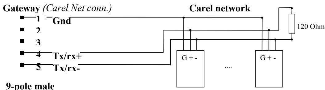
Fig. 7.1.1.1 - Connection in 485
