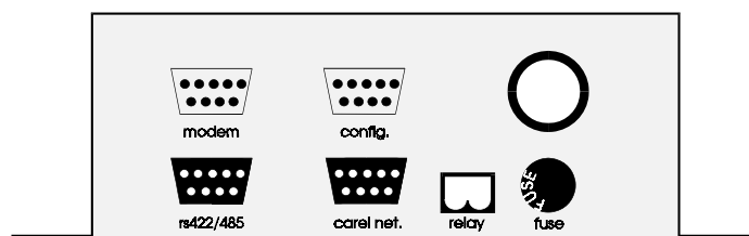
Fig. 2.1 - Gateway back
