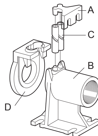
Fig. 7 Foot pedestal
