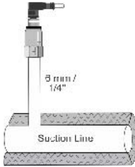
Fig. 5 : PT4-Mxx Series Cable Assembly
