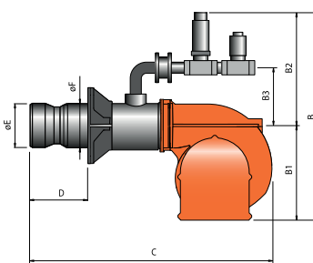
COMIST 180 DSPNM/180 DSPNM-D100
