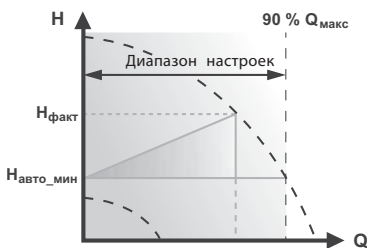
Рис. 32 FLOW_{ADAPT}
