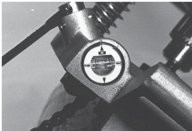
Figure 6 – HC-450 Hole Cutting Tool Level Vial
