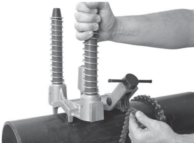
Figure 8 – Hooking the Chain
