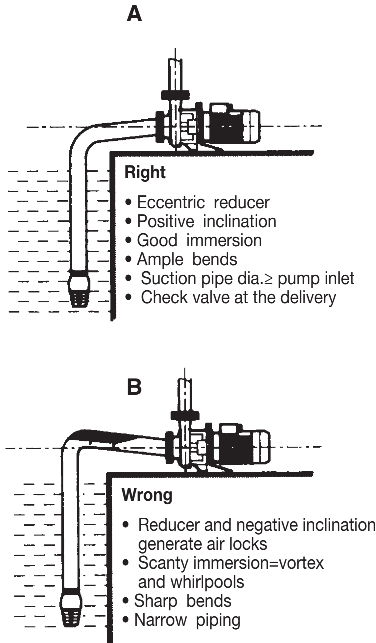
fig. 1 - Pump installation
