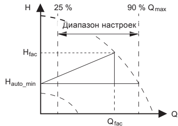
Рис. 37 FLOW ADAPT
