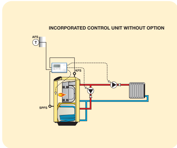
Direct heating circuit with domestic hot water production.
