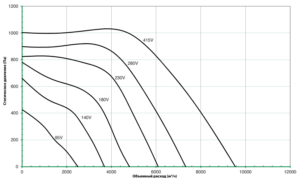
FALCATA 400-4-3
