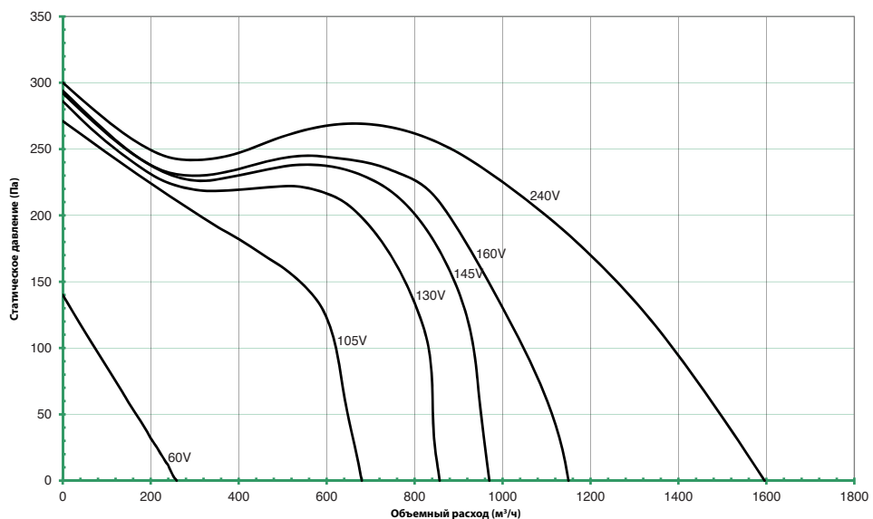
DEBA 200-4-3
