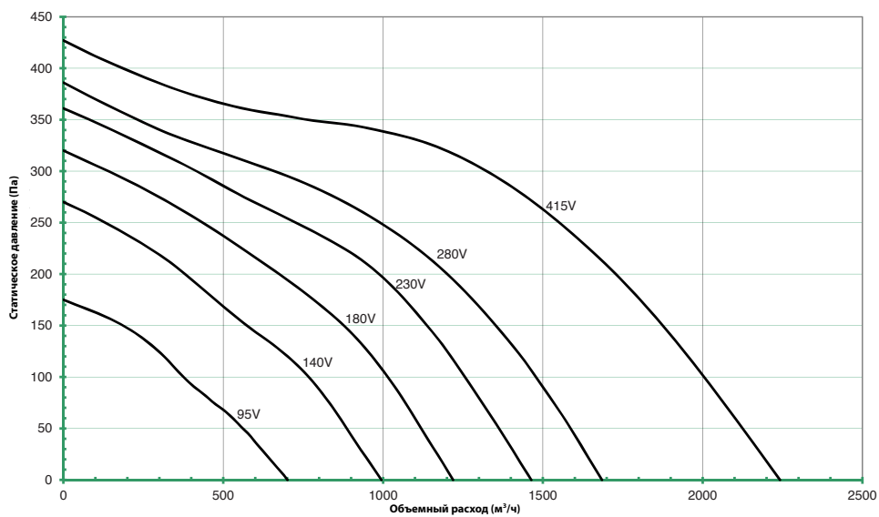
DEBA 225-4-1
