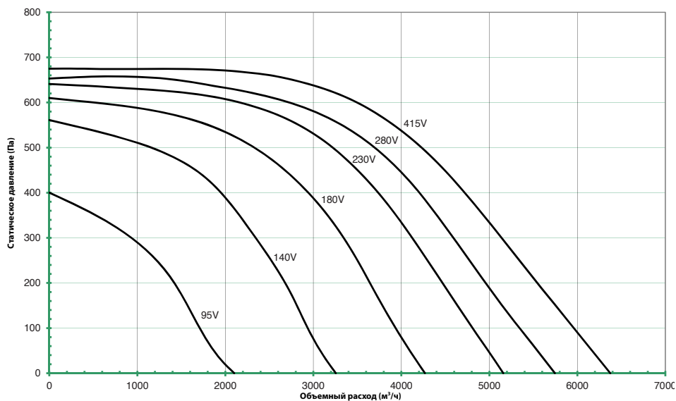
FALCATA 355-6-3
