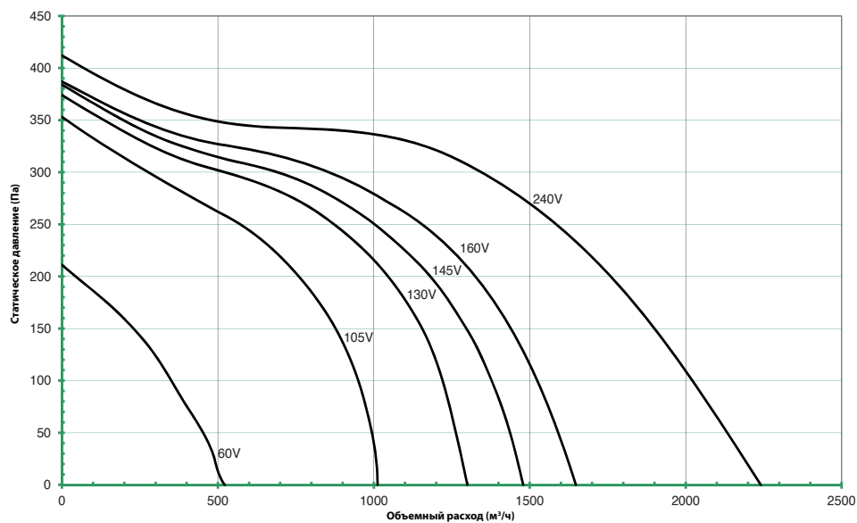
DEBA 225-4-1
