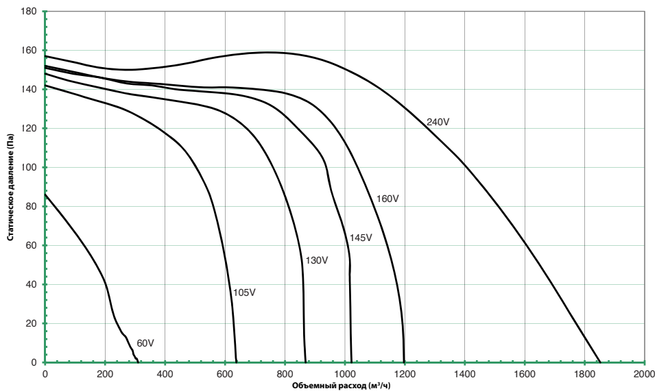
FALCATA 250-4-3
