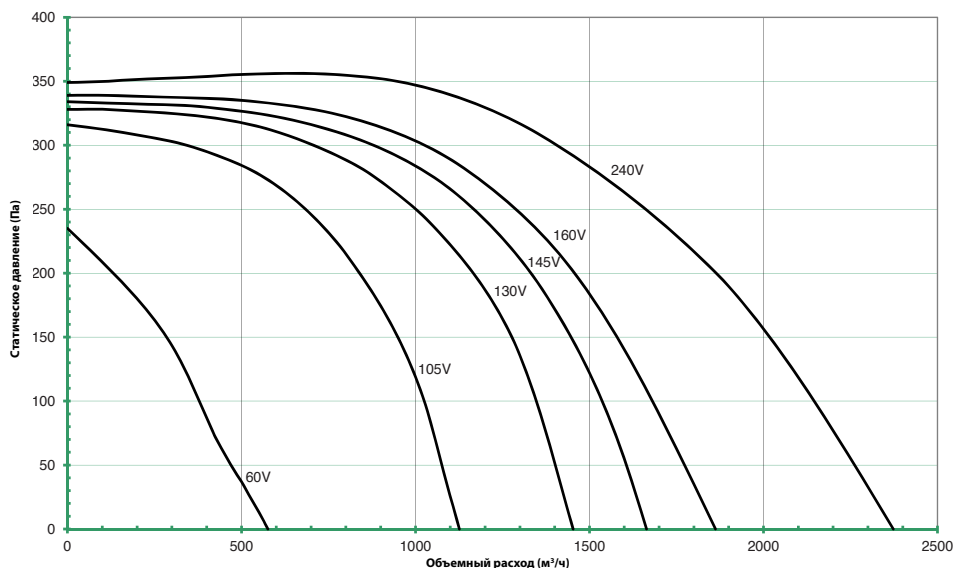
FALCATA 250-4-1
