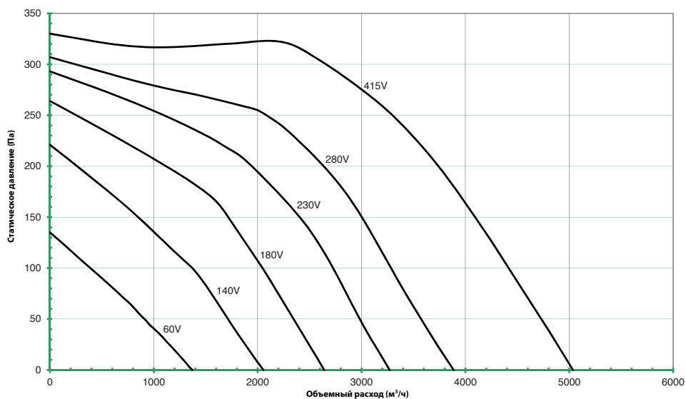
FALCATA 400-4-3
