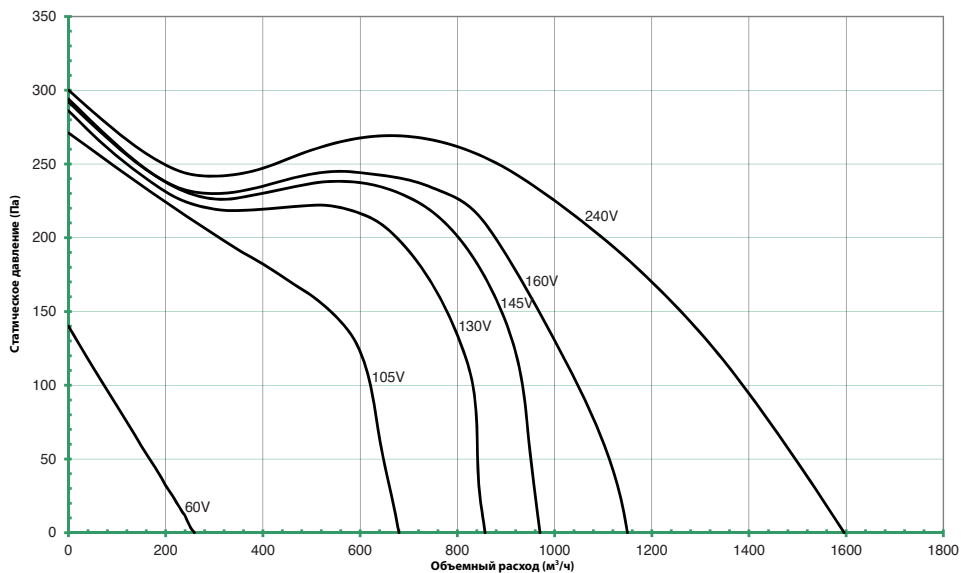
DEBA 225-4-3
