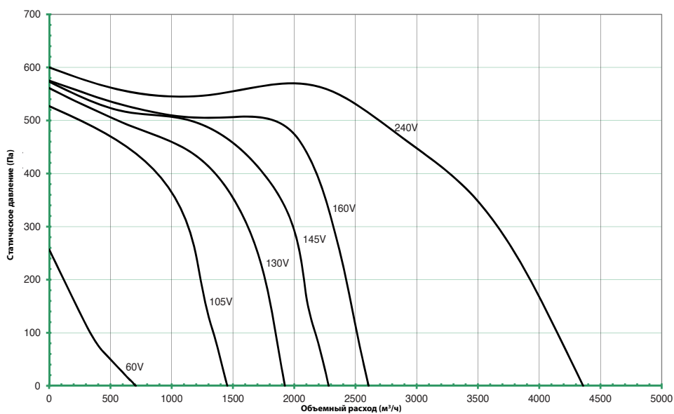
DEBA 280-4-1
