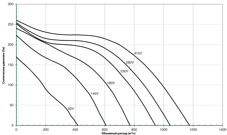
DEBA 180-4-1
