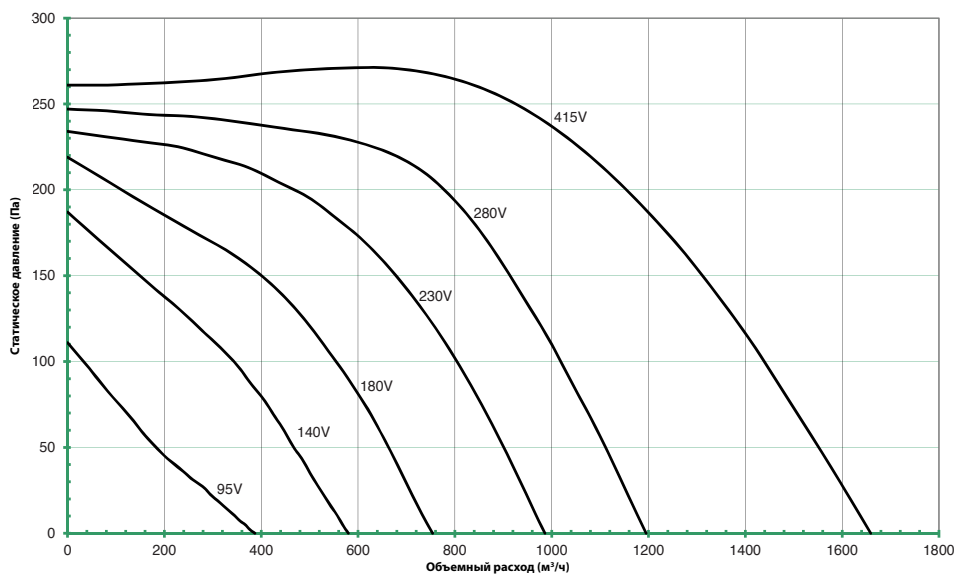
FALCATA 250-4-1
