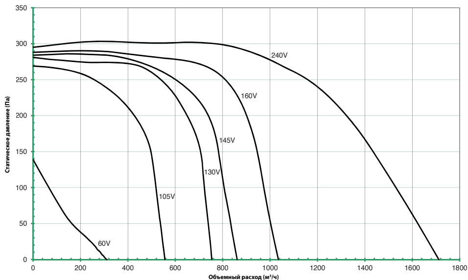
FALCATA 225-4-3
