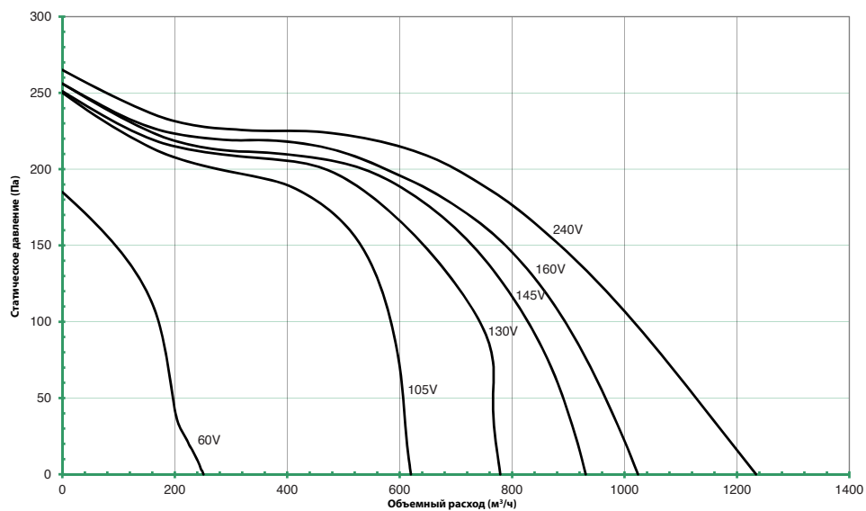
DEBA 200-4-3
