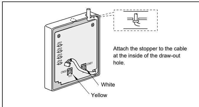
Fig. 6 PCB connector
