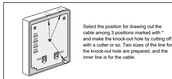
Fig. 5 Drawing out the cable
