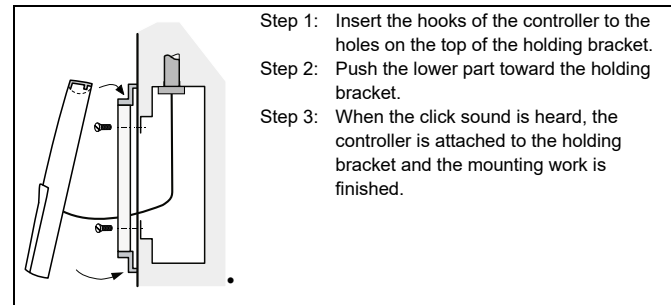
Fig. 10 Mounting procedures
