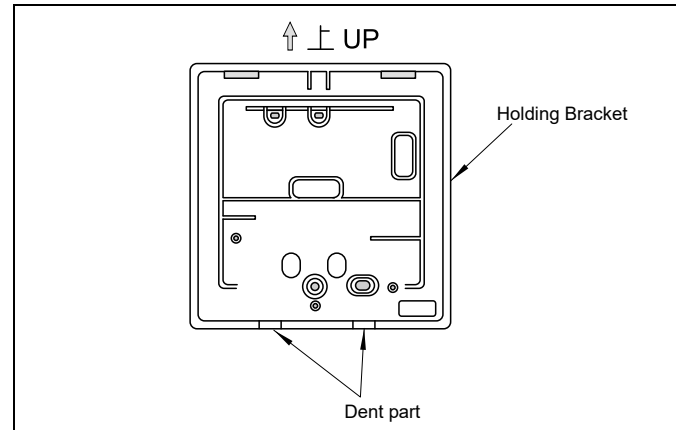
Fig. 3 Installation Procedure
