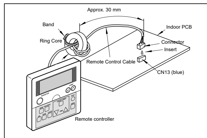
Fig. 12 Electrical Wiring
